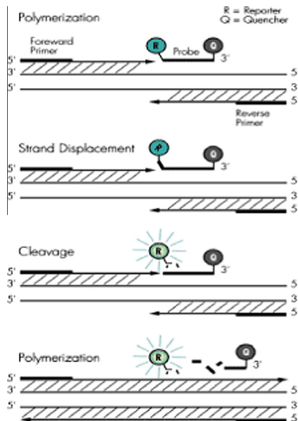
Fig. 1. Principles of real-time PCR Probes**. **Illustration from Heid et al. (1996).
