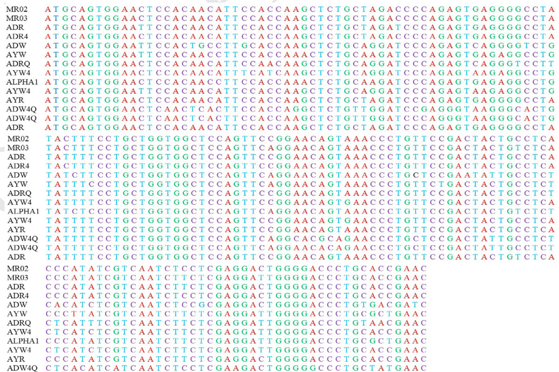
Fig. 2. Alignment of the Pre-S2 region sequences (two samples sequenced in the present study and twelve reported worldwide).
