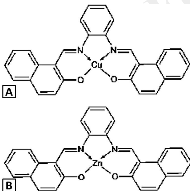
Fig. 1. Structure of test complexes with Schiff base derived ligands: A , NM-3 Tetrakis(2-[(E)-[(2-[(Z)-(2-hydroxynaphthyl)methylidene]amino}phenyl)imino]methyl}phenol)Copper(II). Formula: C 28 H 18 CuN 2 O 2 ; Mol. Wt: 478gms. B , NM-4 Tetrakis (2-[(E)-[(2-[(Z)-(2-hydroxynaphthyl)methylidene]amino}phenyl)imino]methyl}phenol)zinc(II). Formula: C 28 H 18 N 2 O 2 Zn; Mol. Wt: 480gms.
