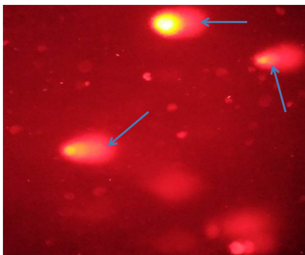
Fig. 1. DNA damage is shown in the form of tail. Arrows pointing to the tails of a damaged DNA.
