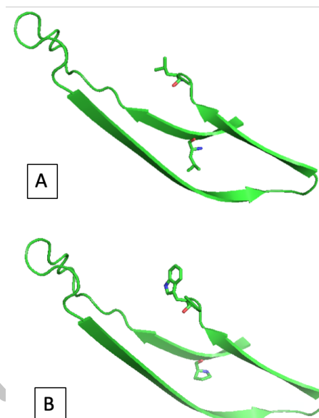
Fig. 2. 3D modeling for the peptide of TNF- \alpha gene of normal (A) and mastitic (B)cows
