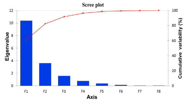
Fig. 1. PCA screen plot showing Eigen values.
