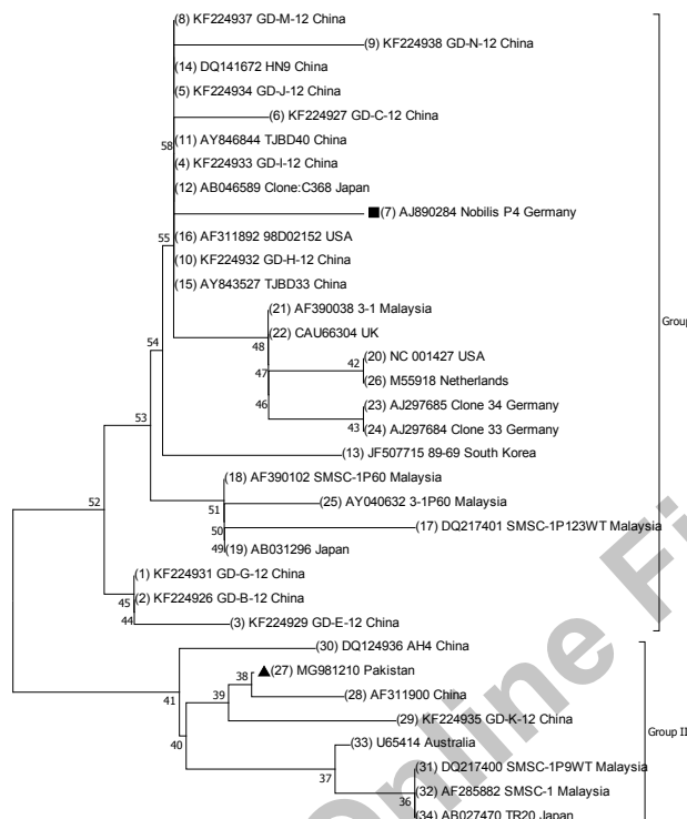
Fig. 1. The phylogenetic tree was inferred by the Neighbor Joining method as described by Saitou and Nei, 1987 . The optimal length of the tree with sum of branch length = 0.11748525 is shown. The tree is sketch to scale having branch lengths in the same units which are used in evolutionary distances to infer the phylogenetic tree. Evolutionary distances were calculated by using the Poisson correction method as mentioned by Zuckerkandl and Pauling (1965) and are in the units of the number of amino acids swipe per site. The analysis is made from thirty-four amino acids sequences. All sites having gaps and missing data were eliminated. There were total 222 positions in final dataset. Evolutionary assessment was carried out in MEGA7 ( Kumar et al., 2016 ).
