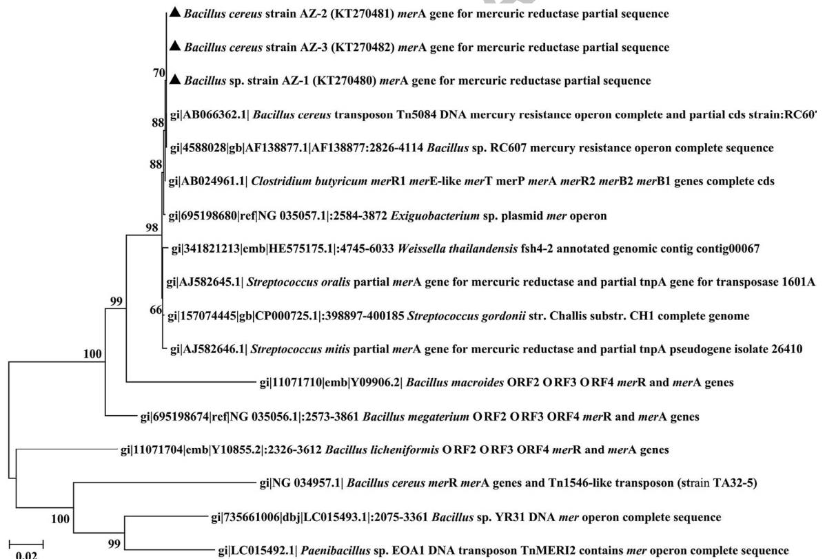
Fig. 2. Evolutionary relationship of different Bacillus sp. on the basis of merA gene was inferred using the Neighbor-Joining method with the sum of branch length 0.53623375. The branch lengths and the evolutionary distances used to infer the phylogenetic tree are in the same units with the bootstrap test value 500. The analysis involved 17 nucleotide sequences and codon positions included were 1st+2nd+3rd+Noncoding. A total of 1279 positions were in the final dataset with no gaps and missing data. Evolutionary analyses were performed by MEGA 5 software (Tamura et al. , 2004).
