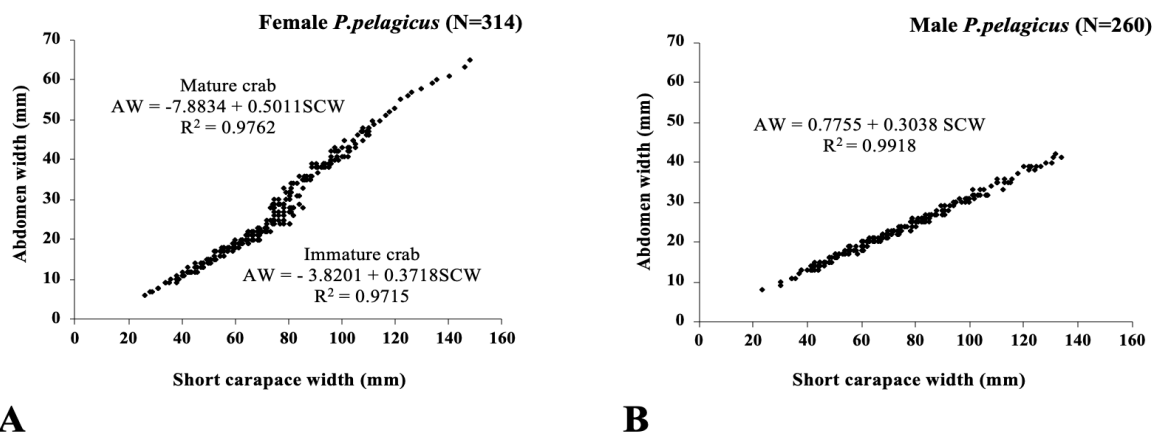
Fig. 3. Relationship between short carapace width (SCW) and abdomen width (AW) in (A) female (N=314) and (B) male (n=260) of Portunus pelagicus .
