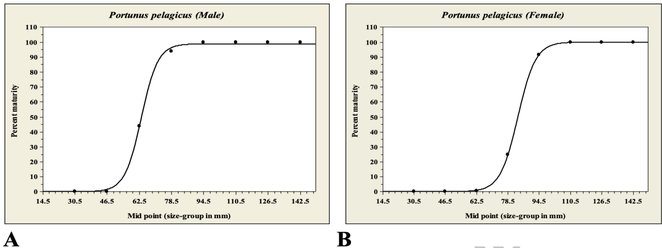
Fig. 4. Size of 50% maturity in different size groups of (A) male (n=941) and (B) female (n=1057) of Portunus pelagicus estimated by evaluating the logistic curve.
