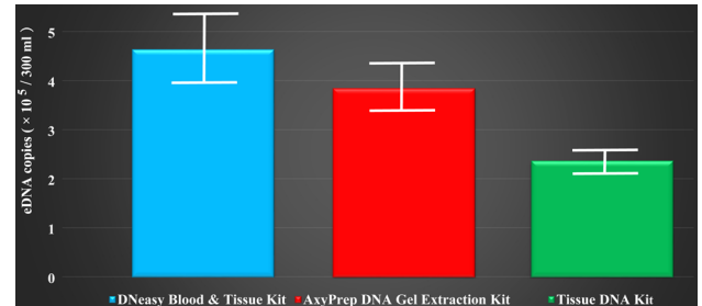
Fig. 3. The DNA yield (copies/300 ml) of Sepiella japonica extracted from aquaculture water (indoors water sample). There was no difference in eDNA yield between the DNeasy Blood and Tissue Kit and AxyPrep DNA Gel Extraction Kit groups ( p=0.061 ).
