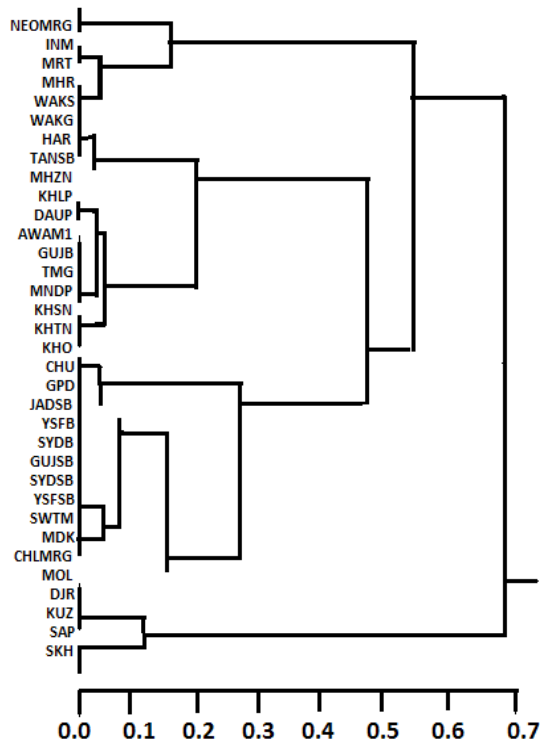
Fig. 2. All samples prehistoric and living central Asians, Pakistanis and peninsular Indians, through hierarchical cluster method.
