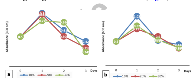
Fig. 1. Effect of inocula sizes on growth of the probiotic isolates Sphingomonas sp. AsCh-P3 (a) and Bacillus aerius AsCh-A7 (b) in fish feed extract (20% w/v) at room temperature for different incubation days.
