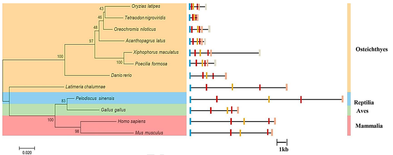
Fig. 3. Phylogenetic relationship and structure of the Almyomaker gene with other vertebrates. Genome structure analysis of Almyomaker genes according to their phylogenetic relationship. Lengths of exons and introns of each Myomaker gene are displayed proportionally. Different colour boxes and lines represent exons and introns, respectively. The identical colour boxes represent homologous sequences.
