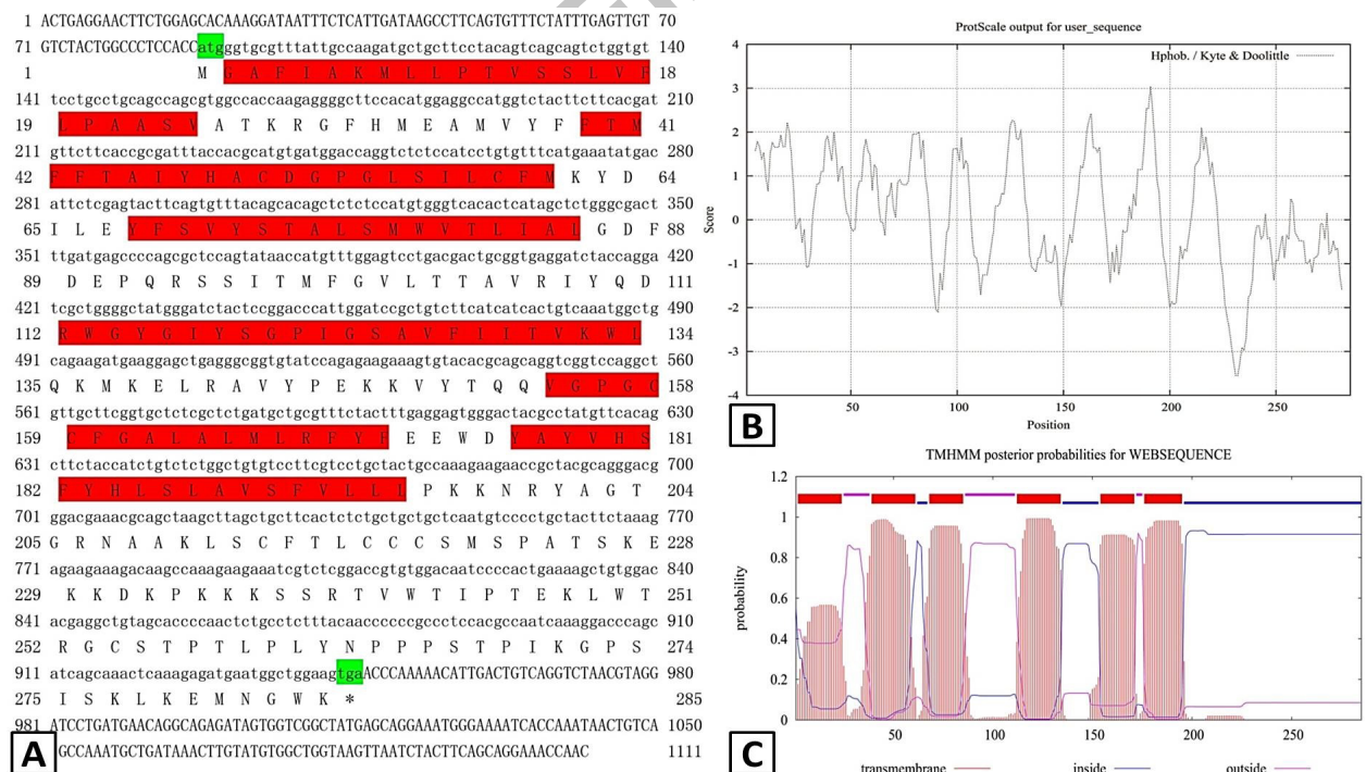
Fig. 1. Sequence characterization of the Myomaker gene in Acanthopagrus latus . A, the nucleotide sequence of the Myomaker gene and the deduced amino acid sequence of T. ovatus . Initiation and termination codons are marked by green. Six transmembrane domains are shown in red; B, hydrophobicity profile of Myomaker ; C, TMHMM posterior probabilities of Myomaker .
