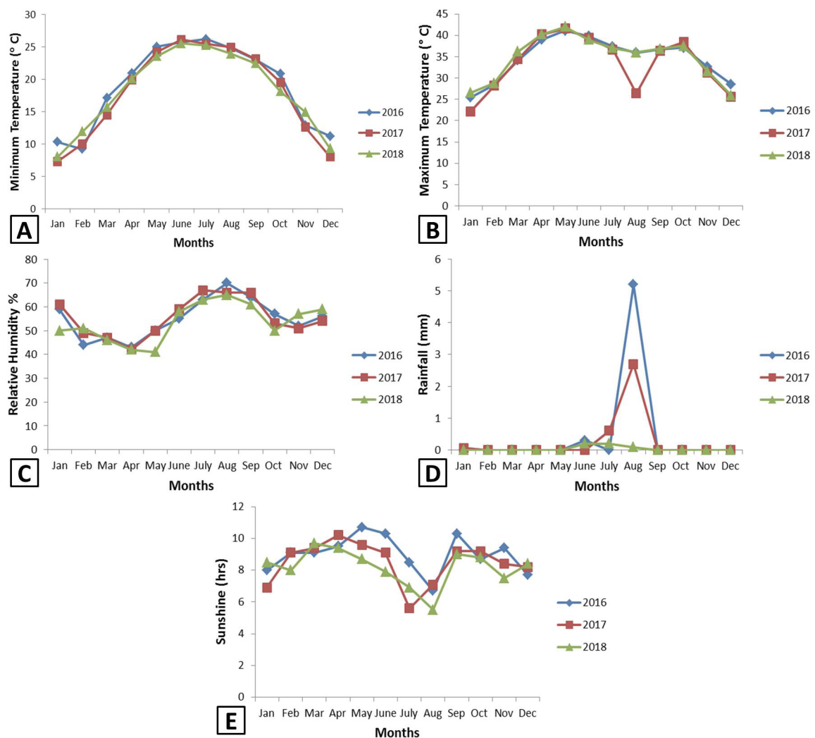
Supplementary Fig. 1. Meteorological data in different months during 2016-2018: A, minimum temperature (°C); B, maximum temperature (°C); C, relative humidity (%); D, rainfall (mm); E, sunshine (h).
