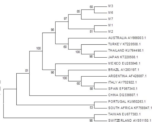
Fig. 2. Nucleotide based tree for MSP4 gene of Anaplasma marginale by Maximum Likelihood Method.
