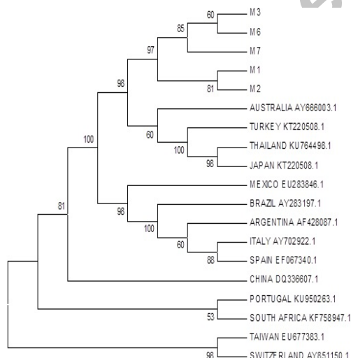
Fig. 1. Nucleotide based tree for msp1a gene of Anaplasma marginale by Maximum Likelihood Method.
