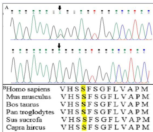
Fig. 3. Chromatogram and Clustal Omega alignment of COL10A1. A , Chromatogram for COL10A1 selected region showing c.2011A>G transition. B , Multiple sequence alignment of COL10A1 from six different organisms performed with Clustal Omega showing p.Ser671Pro (shown in bold) conservation in diverse vertebral species.
