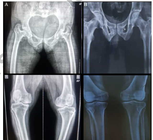
Fig. 2. A , Radiographic features from lower limbs of a metaphyseal chondrodysplasia, Schmid type (MCDS) patient (IV-13 shown in 1B). B , Radiographic features from lower limbs of a normal subject (V-13 shown in 1B). MCDS patient had bowed lower legs, coxa valga, metaphyseal widening and sclerosis while these changes were not observed in control subject.
