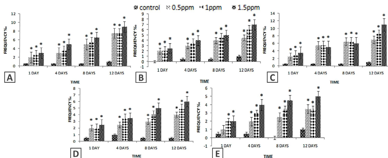
Fig. 1. Effect of chlorpyrifos (A), malathion (B), cypermethrin (C), cyhalothrin (D) and bucril (E) on micro nuclei of haemolymph of Perna viridis .
