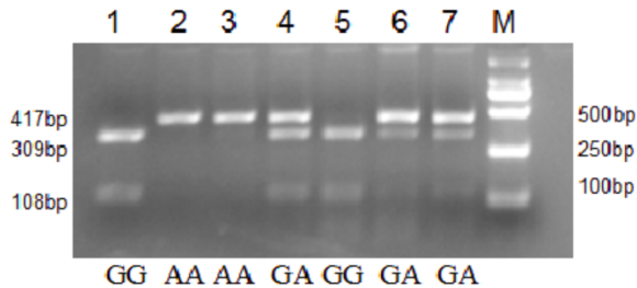
Fig. 2. PAGE map of DHCR24 gene 3'UTR digestion results. Lanes 1-7 show different Chinese Simmental cattle populations in which two bands are GG genotype, three bands are GA genotype and one band is AA genotype.
