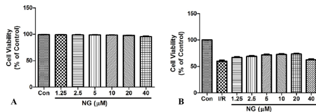
Fig. 1. Effect of naringenin on the cell viability by H/R in H9c2 cardiomyocytes. A) H9c2 cells were treated with various concentration of naringenin for 24 h and MTT assay was used for the estimation of cell viability. B) H9c2 cells were treated with for 12 h with naringenin and then exposed to 6h of hypoxia. The data presented as means \pm SD from three independent experiments.
