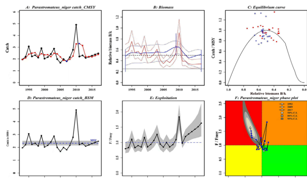
Fig. 5. Estimated results of CMSY and BSM method for Parastromateus niger (A) Time series of catch (black line) and moving average (red line) (B) Relative biomass estimated by CMSY (blue lines) and BSM (red lines) (C) Curve estimated by CMSY (blue dots) and BSM (red dots) (D) Time series catch (E) Exploitation rate (F) Kobe plot of P. niger stock status B/B_{MSY} and fishing mortality ratio F/F_{MSY} indicating (Red= Overfished, Dark yellow = Overfishing, Yellow = Recovering and Green= Safe zone). Blue circles represent the estimated trajectories (1993-2017) of the Black pomfret fishery in WIO, Pakistan. Grey shaded area denotes 50%, 80% and 95% confidence interval. The symbols falling in each quadrant are defined in the legend (right upper corner).
