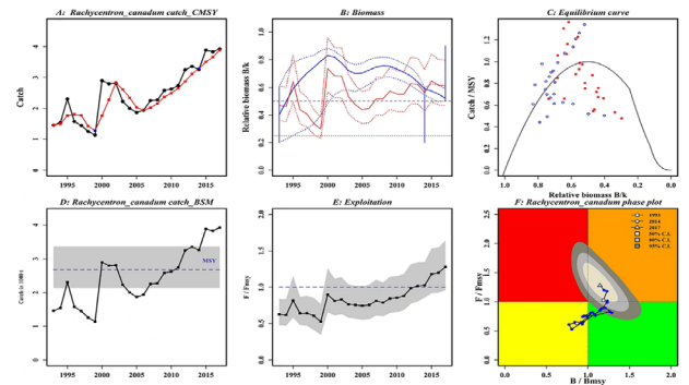
Fig. 4. Estimated results of CMSY and BSM method for Rachycentron canadum (A) Time series of catch (black line) and moving average (red line) (B) Relative biomass estimated by CMSY (blue lines) and BSM (red lines) (C) Curve estimated by CMSY (blue dots) and BSM (red dots) (D) Time series catch (E) Exploitation rate (F) Kobe plot of R. canadum stock status B/B_{MSY} and fishing mortality ratio F/F_{MSY} indicating (Red = Overfished, Dark yellow = Overfishing, Yellow = Recovering and Green = Safe zone). Blue circles represent the estimated trajectories (1993-2017) of the Cobia fishery in WIO, Pakistan. Grey shaded area denotes 50%, 80% and 95% confidence interval. The symbols falling in each quadrant are defined in the legend (right upper corner).
