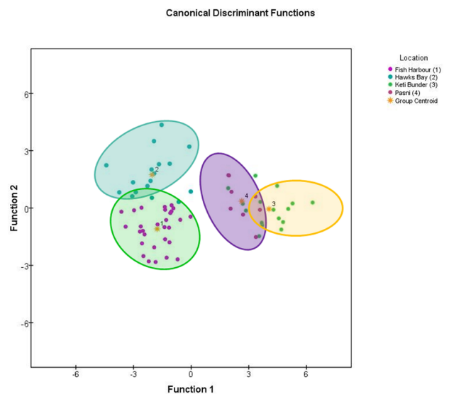
Fig. 4. Canonical discriminant function analysis plotted for goldstripe ponyfish collected from four locations along Pakistani coast using Geo-morphometric variables.
