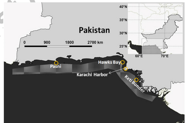
Fig. 1. Sampling locations and coastal fishing grounds of Pakistan are highlighted with shaded area.
