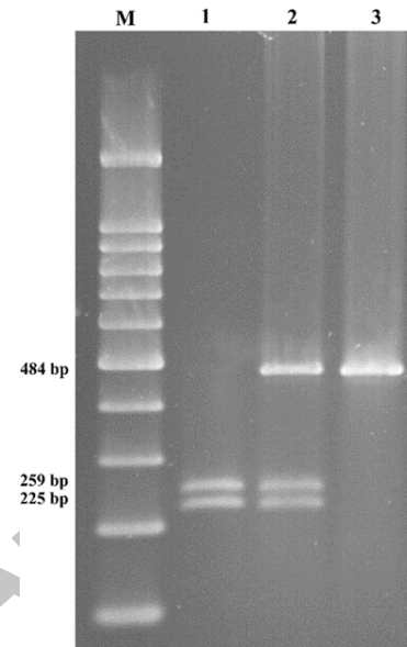
Fig. 2. Agarose gel electrophoresis (2%) of PCR-RFLP of the GSTP1 variant Ile105Val (A to G transition). M lane is 100 bp DNA ladder, Lane 1 contain variant GSTP1 (Val/Val), Lane 2 contain variant GSTP1 (Ile/Val) and Lane 3 contain GSTP1 (Ile/Ile). Band of Fragment of 9 base pairs being very small in size not shown in picture.
