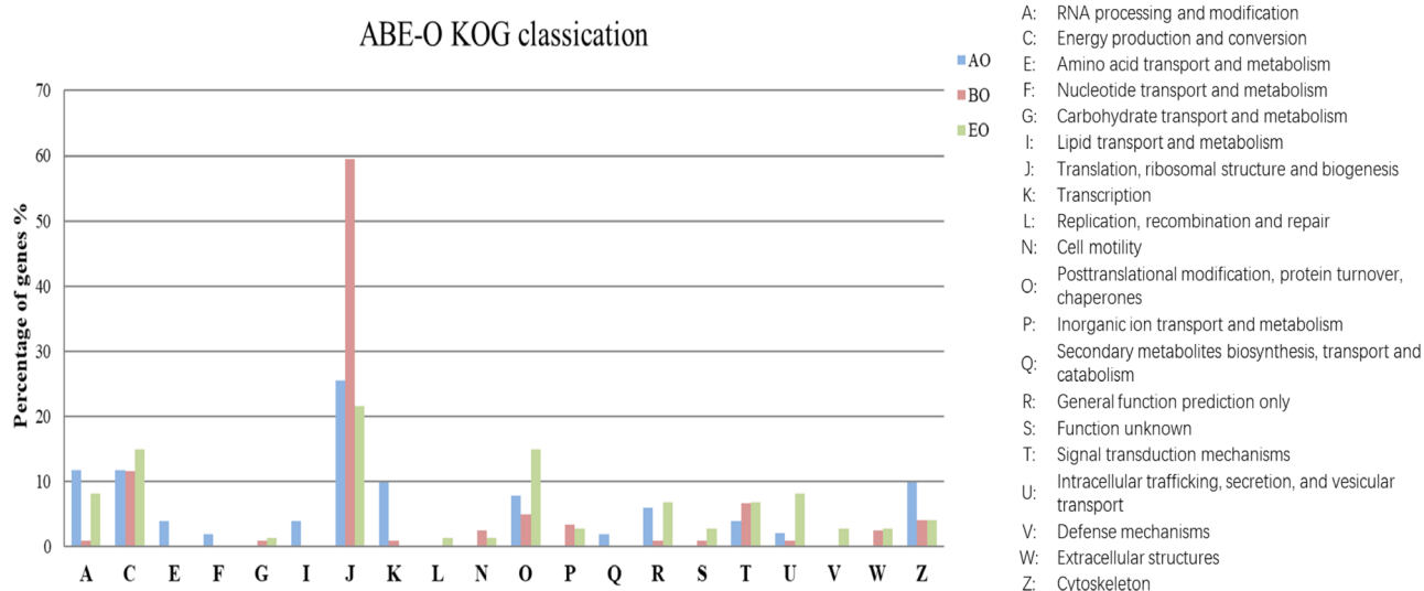
Fig. 3. KOG classification of differential expression genes from the three groups of ovaries. AO, BO and EO represent the three groups in Table II, respectively.
