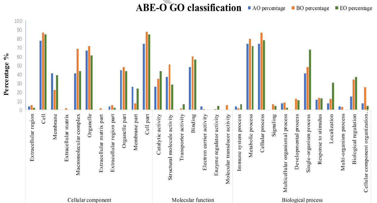
Fig. 2. GO classification of differential expression genes from the three groups of ovaries. AO, BO and EO represent the three groups in Table IV, respectively.
