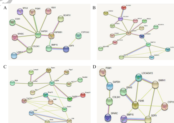
Fig. 6. The relationship prediction between CYP11A1 and efficacy-associated markers among four species. A: cattle; B: human; C: mouse; D: goat.
