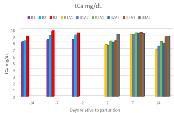
Fig. 3. Means of tCa concentrations for cows fed prepartum and effect of (Tr1) DCAD 0.0, -100, -180 (BC1, BC2, BC3. P < 0.001 ) and effect of postpartum (Tr2) DCAD +250 and +350 (B1A1, B1A2, B2A1, B2A2, B3A1, B3A2. P = 0.511 ), day P < 0.001 and interaction Tr1 x Tr2 x day P = 0.086 , during experimental period.
