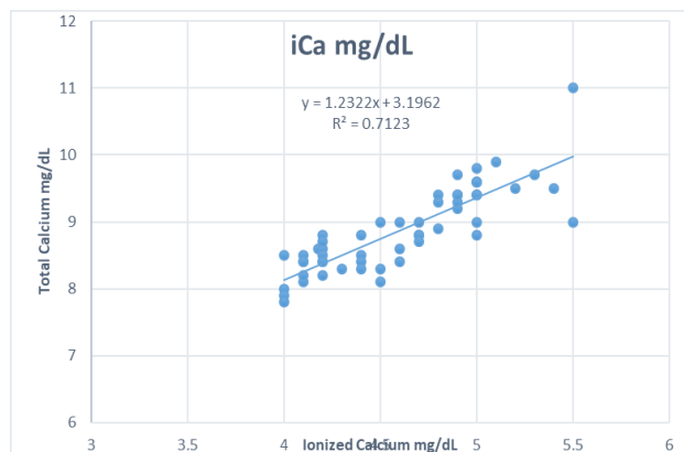
Fig. 5. Simple linear regression and positive correlation between tCa and iCa ( R = 0.84 , R^2 = 0.712 , P < 0.001 ) tCa = 3.2 + 1.23 \cdot iCa for cows fed prepartum (Tr1) DCAD (0.0, -100, -180) there is positive linear relationship tCa and iCa p < 0.05 .
