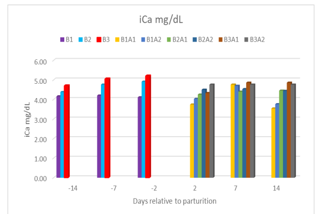
Fig. 4. Means serum iCa concentrations for cows fed prepartum and effect of Tr1 DCAD 0.0, -100, -180 (BC1, BC2, BC3. P < 0.001 ) and effect of postpartum Tr2 DCAD +250 and +350 (B1A1, B1A2, B2A1, B2A2, B3A1, B3A2. P = 0.511 ), day P < 0.001 and interaction Tr1 x Tr2 x day P = 0.510 , during experimental period.
