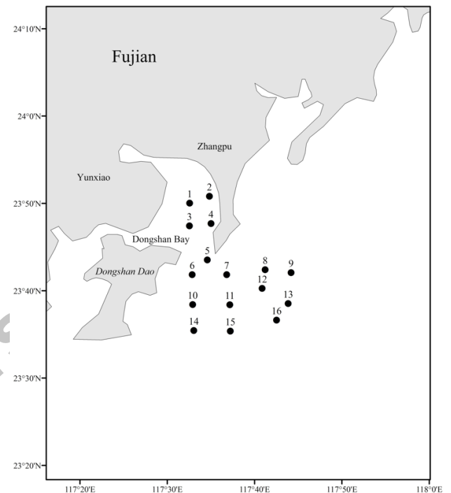
Fig. 1. Distribution of survey stations in Dongshan Bay.
