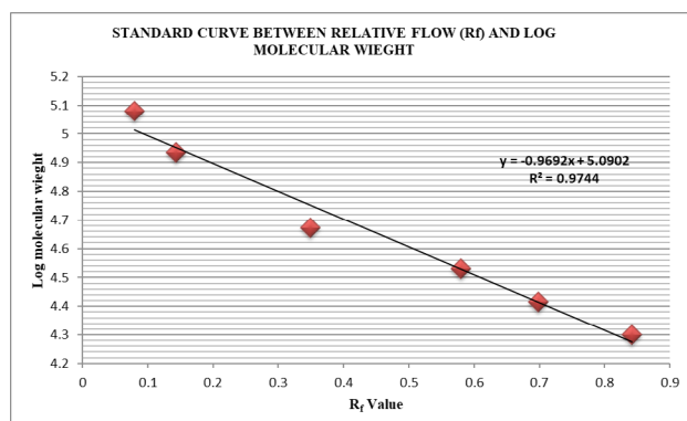
Fig. 4. A standard Curve obtained by plotting a scatter graph between Rf values and log of known molecular weight of protein marker. The X-axis shows the Rf values ranging from 0 to 0.9. Y-axis shows the log of molecular weight ranging from 4.2 to 5.2. The regression formula ( y = -0.9692x + 5.0902 ) obtained was used to calculate the molecular weight of all the unknown proteins separated on the gel. Where Y= Rf value of that specific protein band and X= Molecular weight of unknown protein band.
