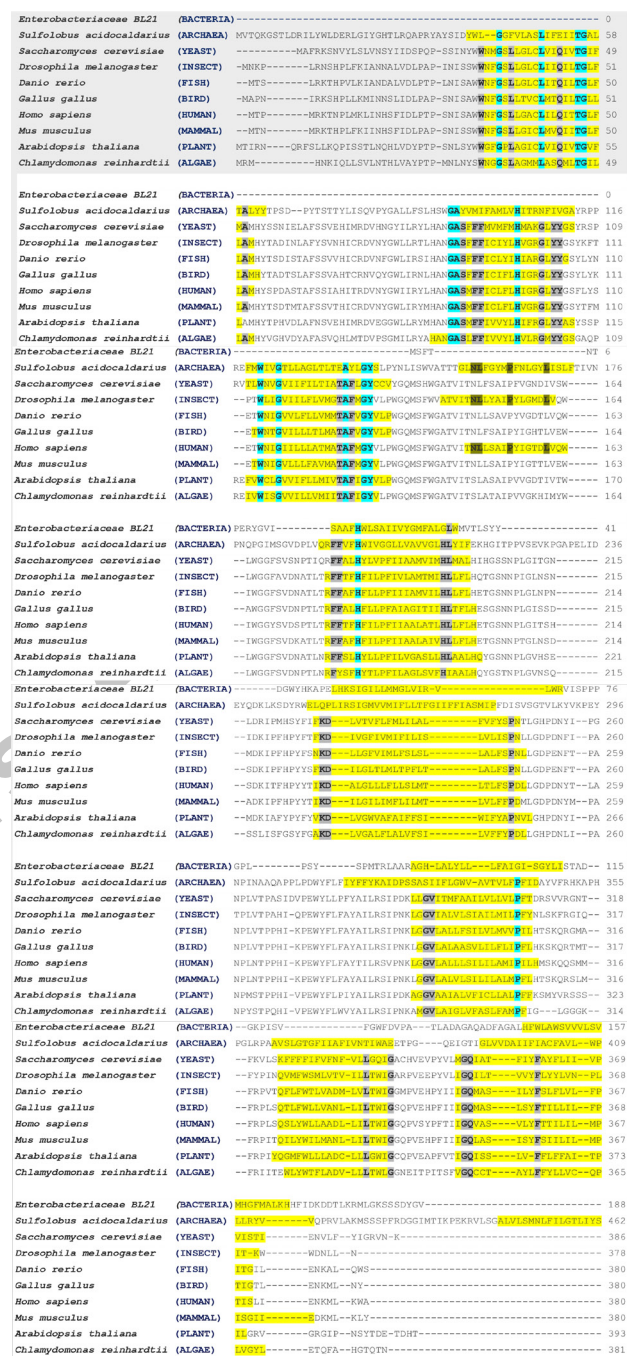
Fig. 8. Multiple sequences alignment of cytochrome b protein in the model organism. Transmembrane alpha-helices in model organisms are highlighted in yellow colour. The conserved residues in archaea and eukaryotic are highlighted with turquoise colour. The eukaryotic conserved residues are highlighted with Gray colour. The dark yellow colour indicates the conserved residues in the high number of transmembrane alpha-helices model organisms. The MSA were performed through the online available Clustal Omega tool ( https://www.ebi.ac.uk/Tools/msa/clustalo ).
