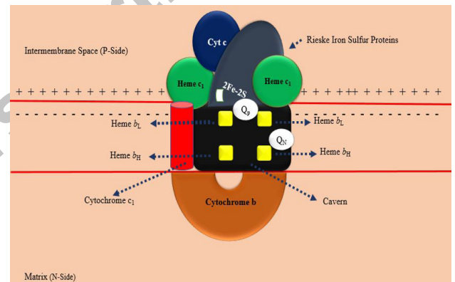
Fig. 2. Structure of mitochondrial cytochrome b in bc_1 complex (drawn by the authors).
