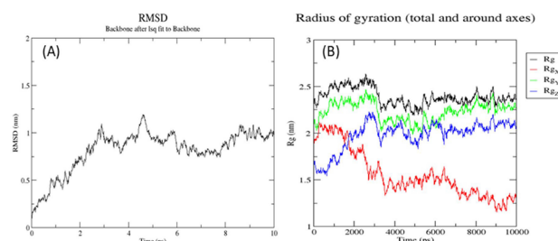
Fig. 9. Root mean square deviation (RMSD) (A) and radii of gyration (B) of 3D predicted structure of ZntR protein.
