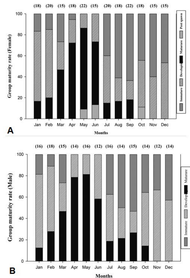
Fig. 4. Monthly variations in the group maturity rate for silver pomfret in the Bay of Bengal.
