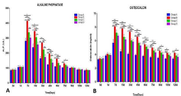
Fig. 4. Changes in alkaline phosphatase (A), osteocalcin (B) in each group with time points. For alkaline phosphatase and osteocalcin, significant difference of values i.e., * ( P \leq 0.05 ), ** ( P \leq 0.01 ) of groups A, B, C and D was noted at marked days.
