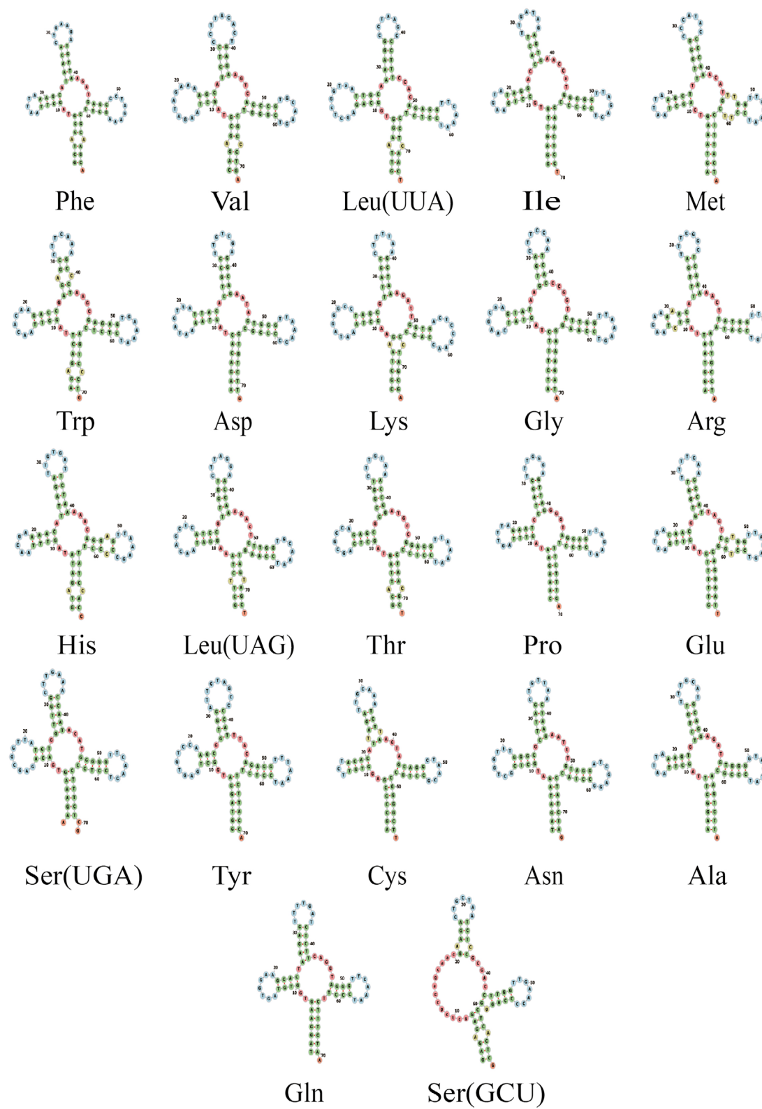
Fig. 4. The presumptive secondary structures of 22 tRNAs in mitochondrion of A. cernua .
