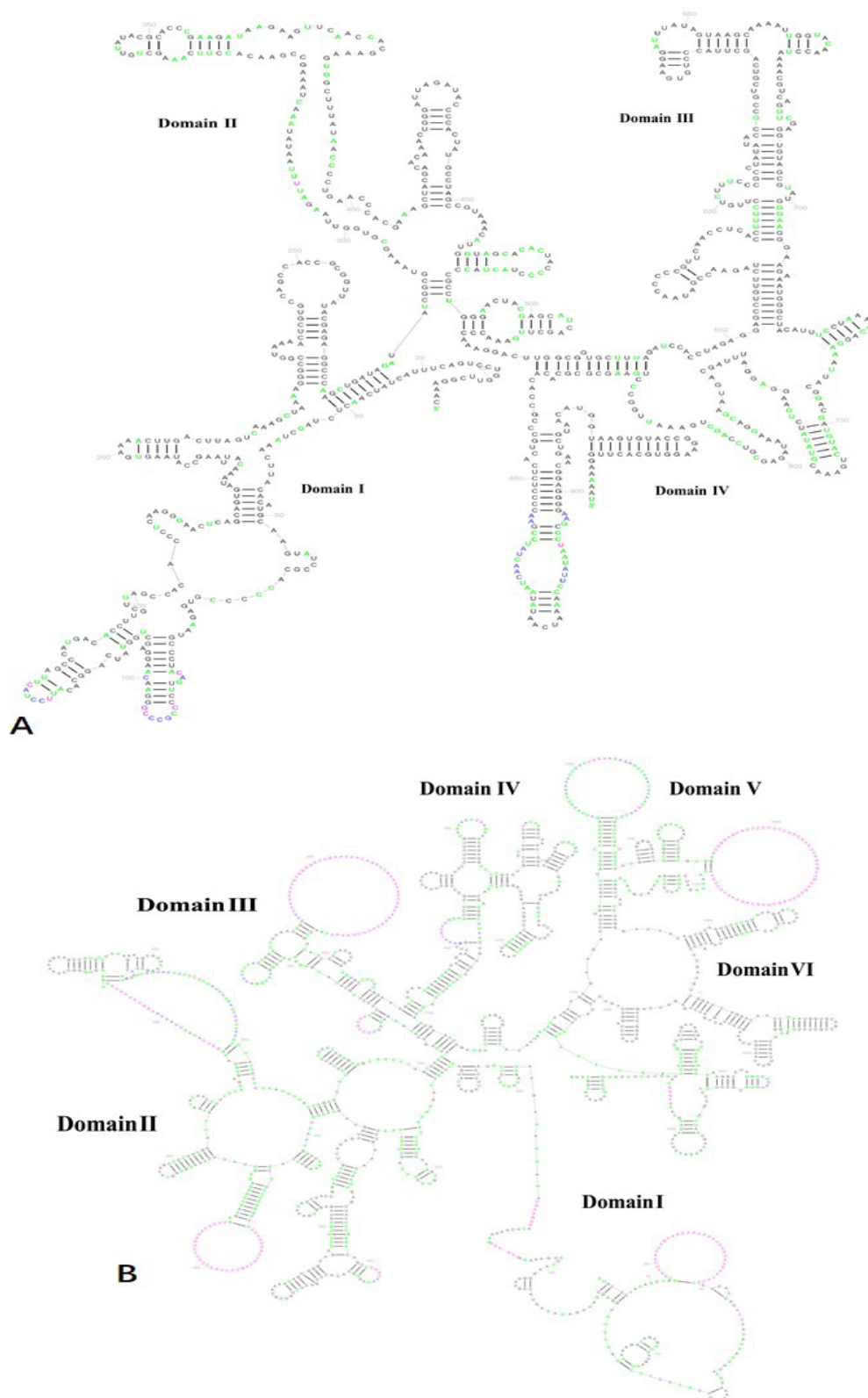
Fig. 5. A: Predicted secondary structure of 12S rRNA (A) and 16S rRNA (B) of A. cernua .
