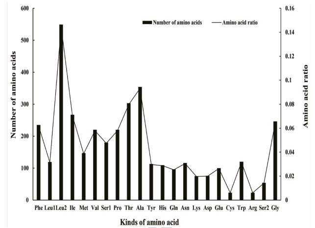
Fig. 3. Quantities of amino acids encoded by PCGs.
