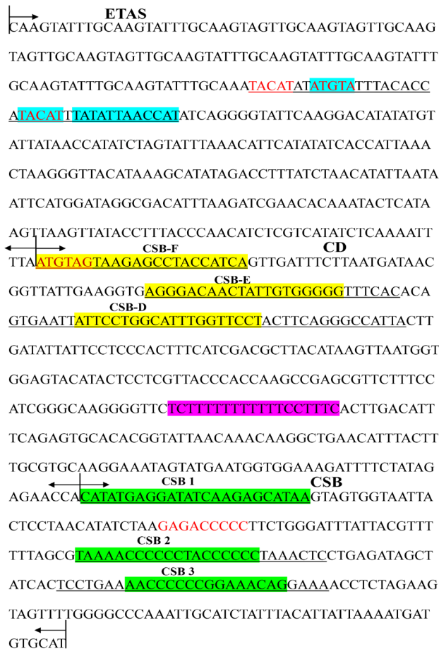
Fig. 6. Mitochondrial control region structure of A. cernua .
