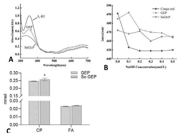
Fig. 4. The \text{I}_2 -KI test of GEP and Se-GEP (A), the maximum absorption wavelength of Congo red test at various concentrations of NaOH (B), and the periodate consumption and formic acid formation of GEP and Se-GEP during periodate oxidation (C). CP, consumption of periodate, FA, formic acid formation.
