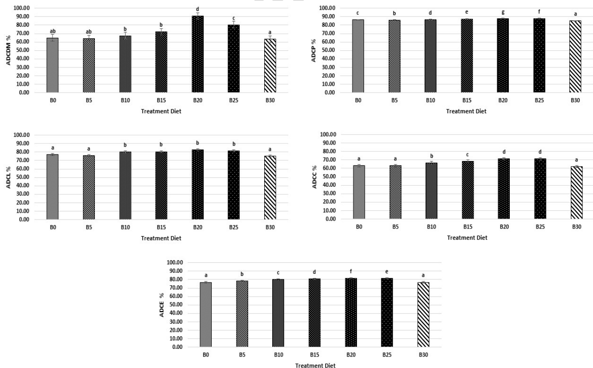
Fig. 3. Apparent digestibility coefficient for dry matter (ADCDM), for protein (ADCP), for lipids (ADCL), for carbohydrates (ADCC) and gross energy (ADCE) of L. rohita . Different alphabets on bars in the same graph indicate statistically significant differences.
