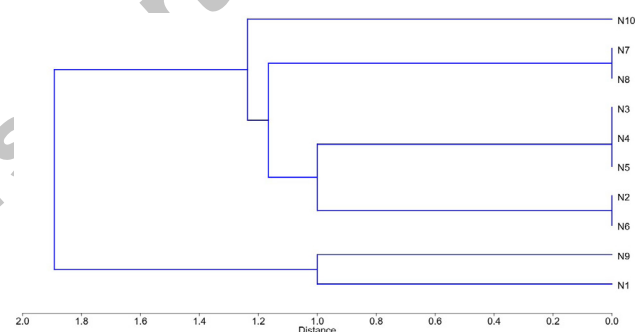
Fig. 4. Phylogenetic tree based on 16S rRNA gene sequencing. For details of isolates N -N 10 , see Table I.
