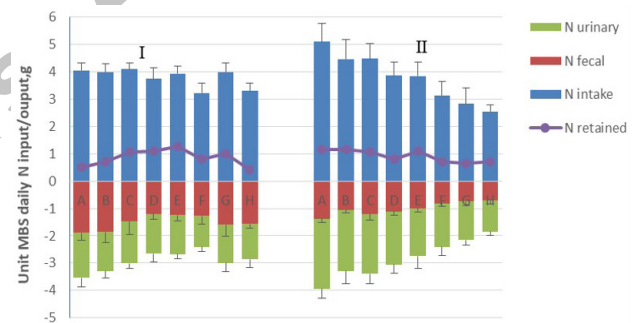
Fig. 2. N input/output relationships for mink, values are means and SD.
