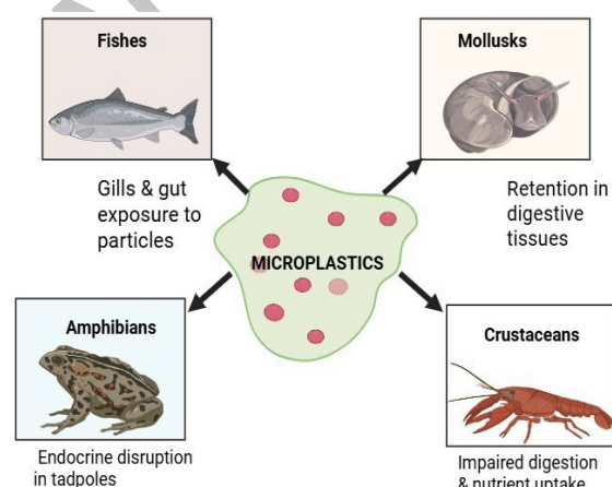
Fig. 2. Ingestion by aquatic fauna. Pathways of MP uptake in aquatic organisms.
