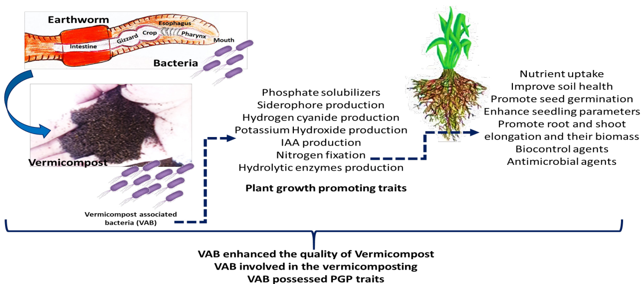
Supplementary Fig. 1. Production and importance of vermicompost associated bacteria as plant growth promoting bacteria.
