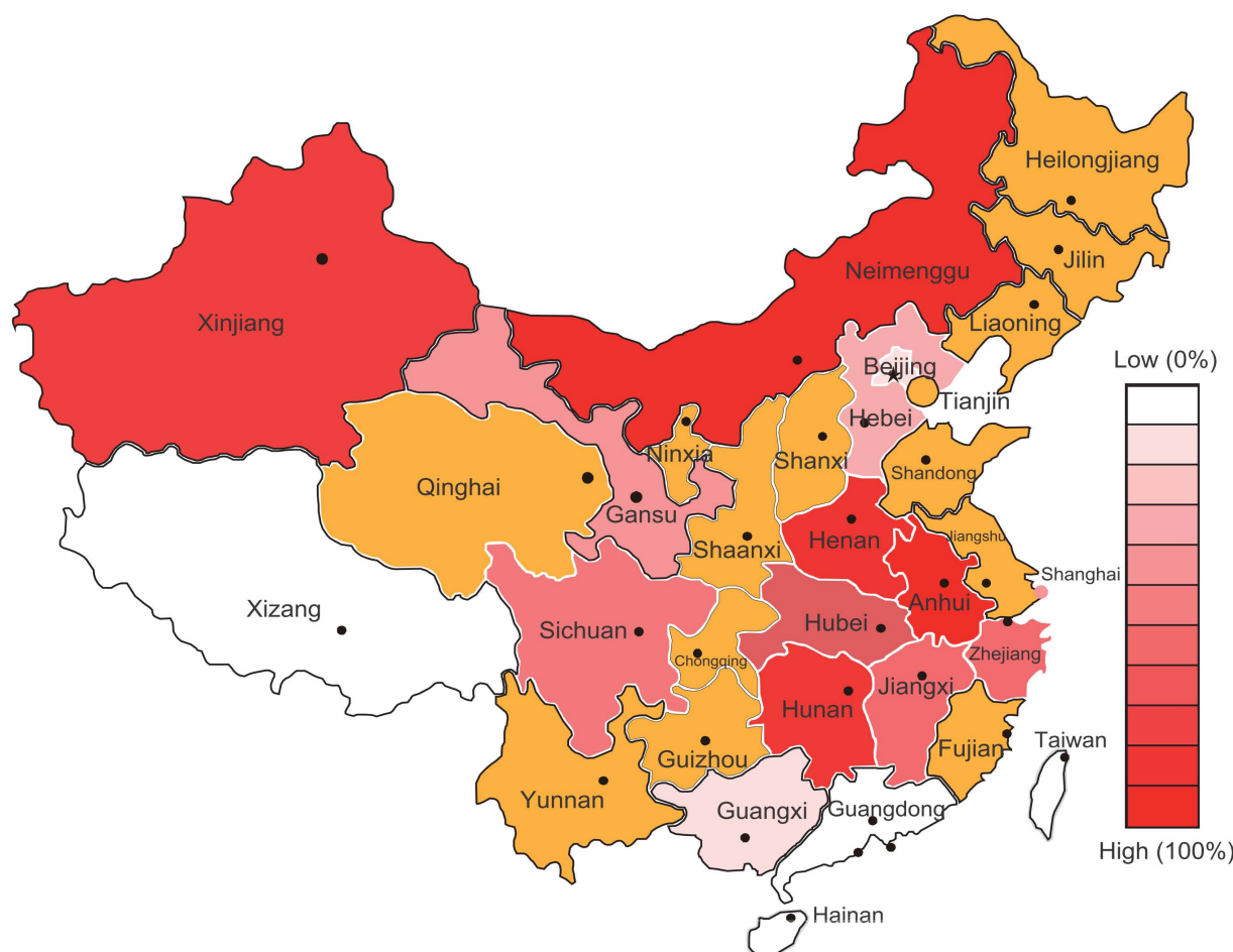
Fig. 1. Distribution of Aichivirus C in China. Different shades of red colour indicate various-total infection rates of Aichivirus C in porcine faeces and intestine samples. Light red to dark red colours are corresponding to 0% to 100% Aichivirus C infection rates. For districts where no literature has been reported, the presence of Aichivirus C is indicated by no colour. Districts in orange indicate Aichivirus C exists in this region, but currently the prevalence rate is unclear.
