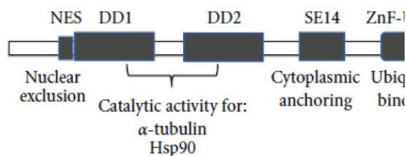
Figure 3. HDAC6 functional domain
