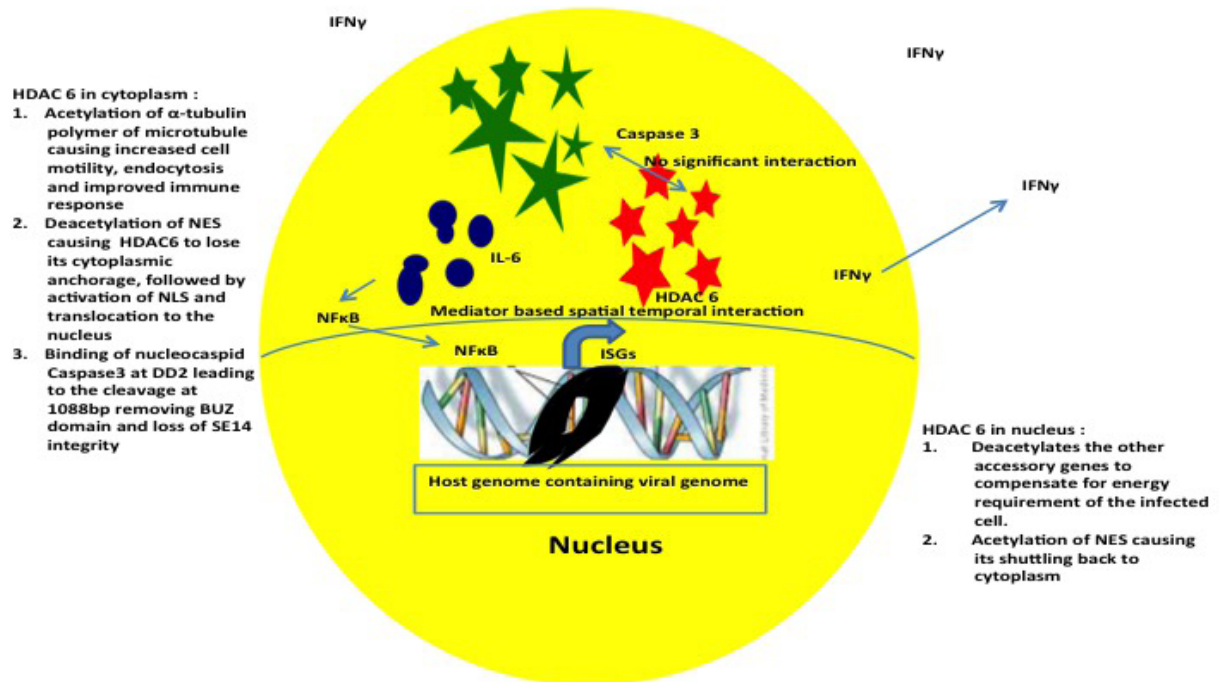
Figure 11. Cascade of events post Viral infection inside the nucleus and production of IFN beta.
