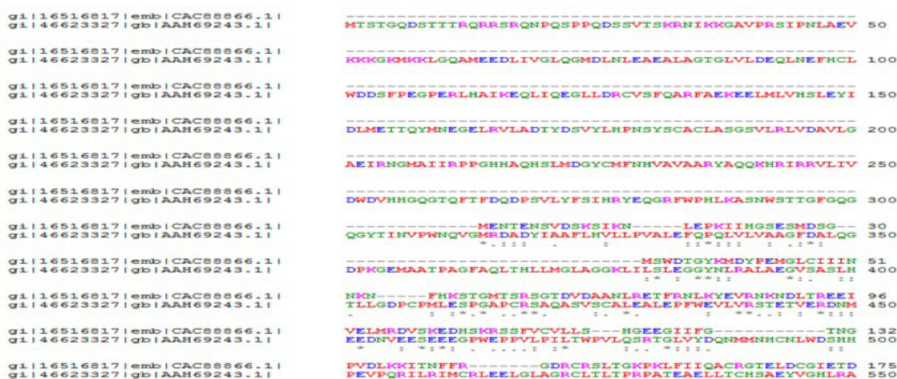
Figure 6. CLUSTALW between HDAC-6 and Caspase 3.
