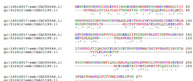
Figure 7. CLUSTALW between IL-6 and Caspase 3.
