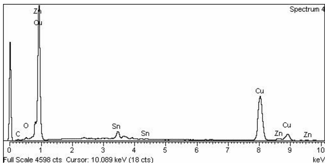
Figure 3: EDX spectrum of a gun metal. Copper, zinc and tin are identifiable
