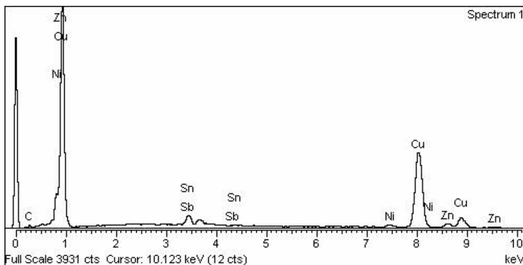
Figure 4: EDX spectrum of gear bronze sample. Copper zinc, nickel, and tin are identifiable
