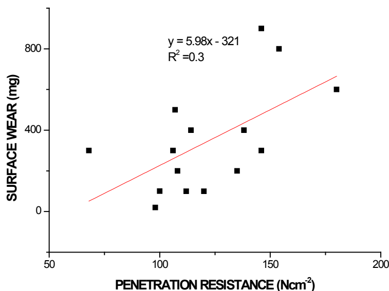
Figure 5: Effect of Soil Resistance on surface wear of gear composition
