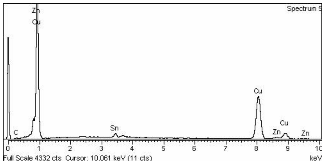
Figure 2: EDX spectrum of a Commercial gun metal sample, copper, zinc and tin are identifiable
