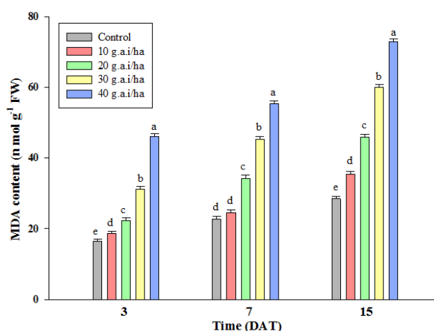
Figure 1: Changes in MDA content (nmol g -1 FW) at various growth stages in Brassica juncea L. cv. alankar exposed to different concentrations of imidacloprid
