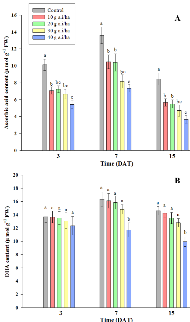
Figure 7: Variations in ascorbate content at various growth stages in Brassica juncea L.cv. alankar treated with different concentrations of imidacloprid. (A) Ascorbic acid (ASC) content (μmol g -1 FW) and (B) dehydroascorbate (DHA) content (μmol g -1 FW). Values with different small letters at each time point are significantly ( p < 0.05 ) different from each other (Duncan's multiple-range test). The values represent Mean \pm SE ( n = 4 ).
