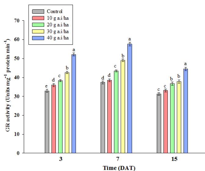
Figure 6: Changes in GR activity (Units mg -1 protein min -1 ) at various growth stages in Brassica juncea L. cv. alankar exposed to different concentrations of imidacloprid
