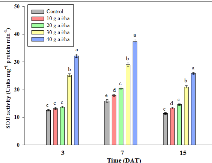
Figure 3: Changes in SOD activity (Units mg -1 protein min -1 ) at various growth stages in Brassica juncea L. cv. alankar exposed to different concentrations of imidacloprid
