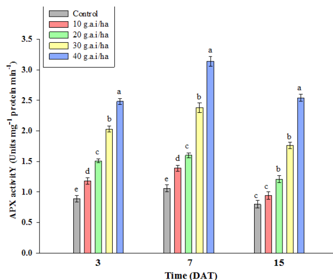
Figure 5: Changes in Apx activity (Units mg -1 protein min -1 ) at various growth stages in Brassica juncea L. cv. alankar exposed to different concentrations of imidacloprid
