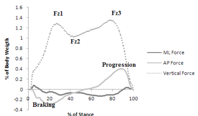
Figure 1: The peaks of the forces selected in this study
