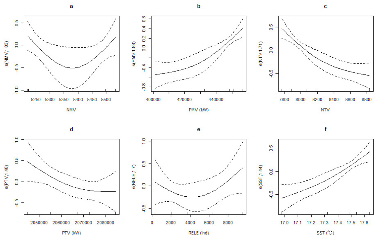
Fig. 3. Impact of (a) the number of main catch vessel (NMV), (b) the power of main catch vessel (PMV), (c) the number of trawl vessel (NTV), (d) the power of trawl vessel (PTV), (e) the release number of larval crab (RELE), and (f) the sea surface temperature (SST) on the catch of Portunus trituberculatus in the northern East China sea.
