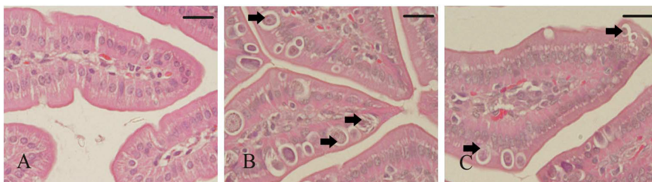
Fig. 1. S. persica reduced change in E. papillata parasitic stages. A, uninfected control jejunum; B, infected jejunum containing developmental stages (arrows); C, Infected treated mouse jejunum (300 mg/Kg) with reduced numbers of developmental stages. Sections were stained with hematoxylin and eosin. Bar=20 \mu m.
