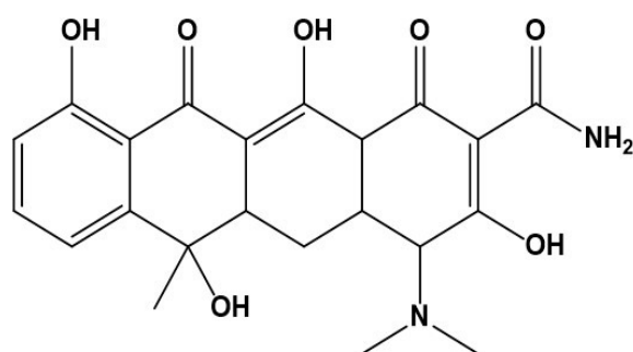
Tetracycline (TET)
