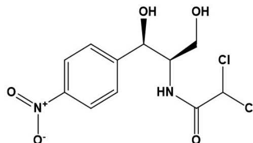
Chloramphenicol (CAP)
