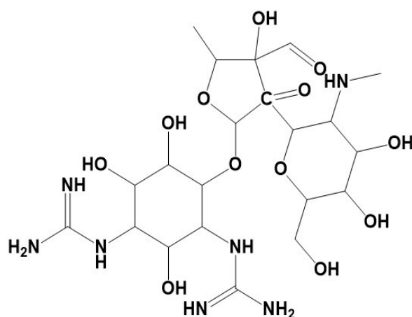
Streptomycin (STR)
