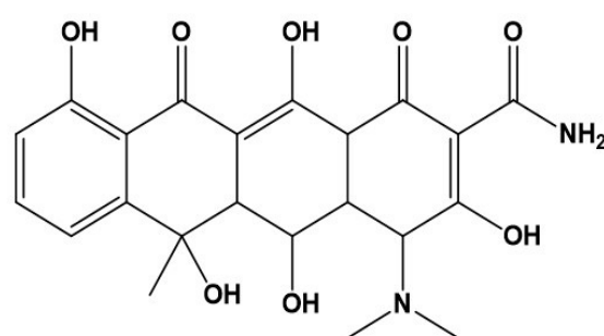
Oxytetracycline (OTC)
