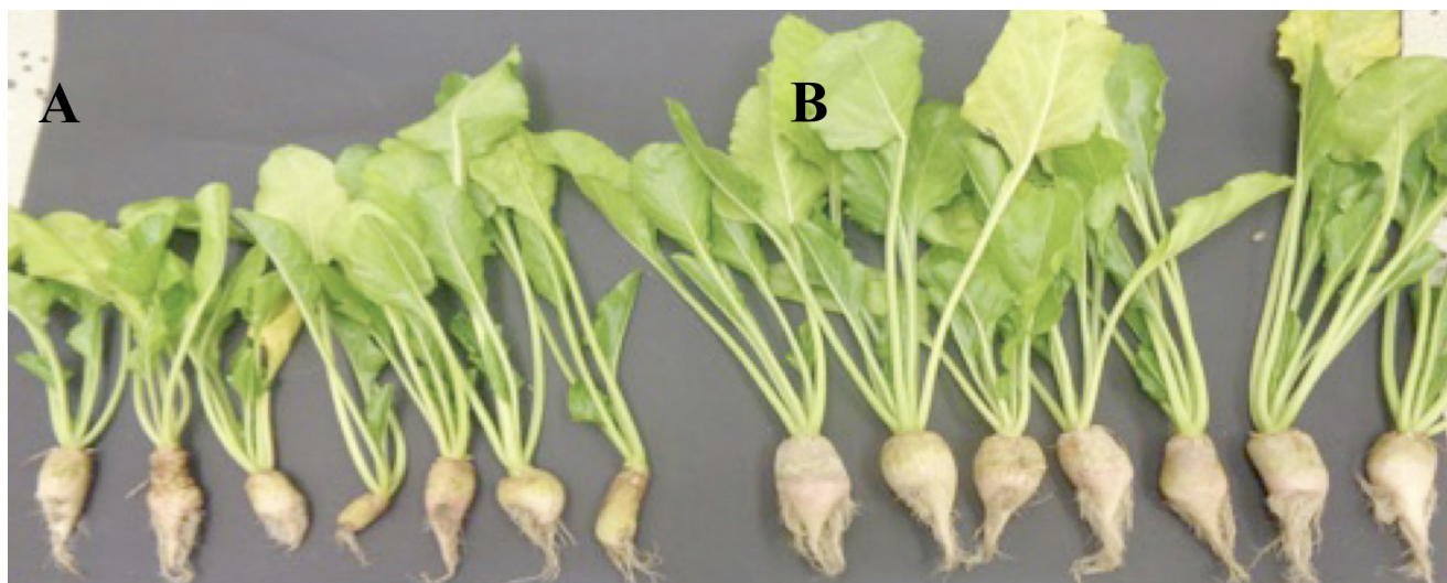
Fig. 2. Comparison of the growth between sugar beet plants treated with (A) Heterodera schachtii alone (control) and (B) together with nematophagous fungus, Lecanicillium muscarium and Heterodera schachtii .
