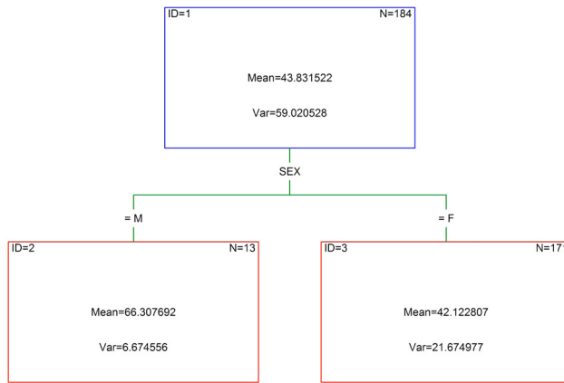
Fig. 1. The layout of CART
