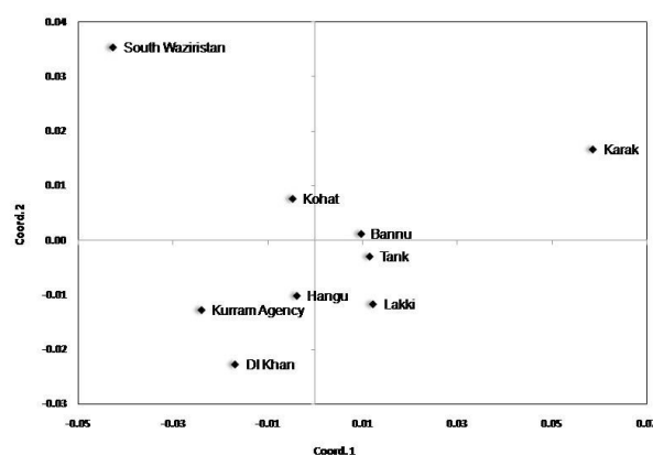
Fig. 2. Scatter plot depicting the output of Principal Component Analysis based on genetic distance matrix in the Pashtun populations.
