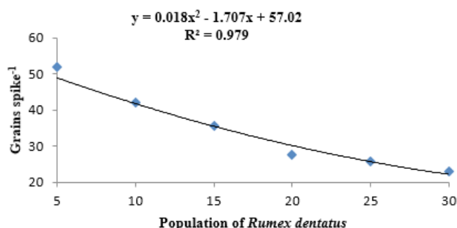
Figure 5: Grains spike -1 as affected by various population of Rumex dentatus
