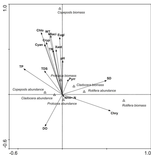
Fig. 6. CCA biplot of environmental factors, phytoplankton and zooplankton communities.
